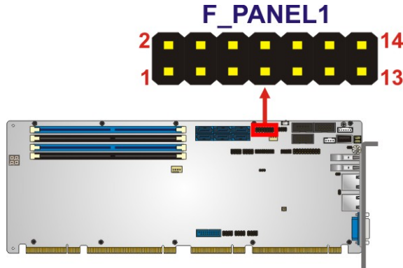
Figure 3-11: Front Panel Connector Location
