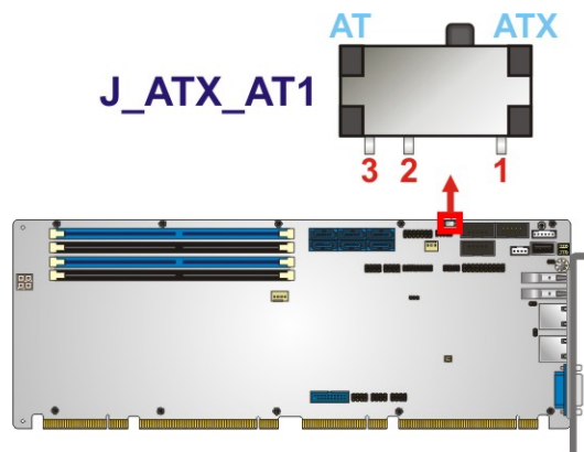
Figure 4-7: AT/ATX Power Mode Switch Location
