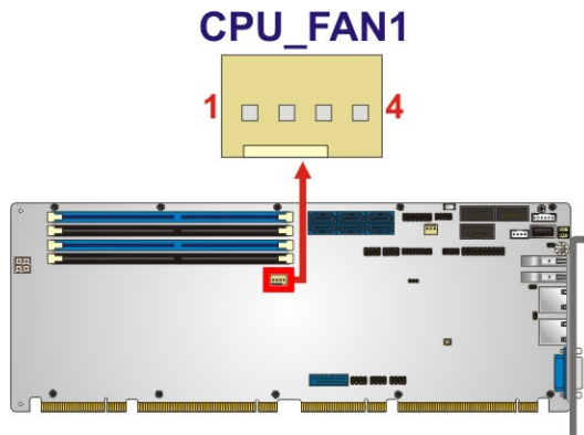
Figure 3-9: CPU Fan Connector Location
