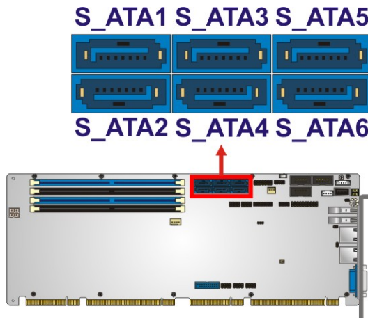
Figure 3-19: SATA 6Gb/s Drive Connector Locations
