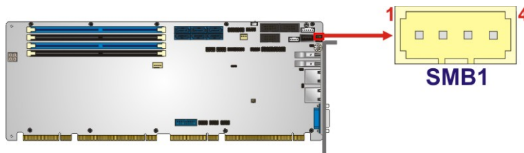
Figure 3-20: SMBus Connector Location
