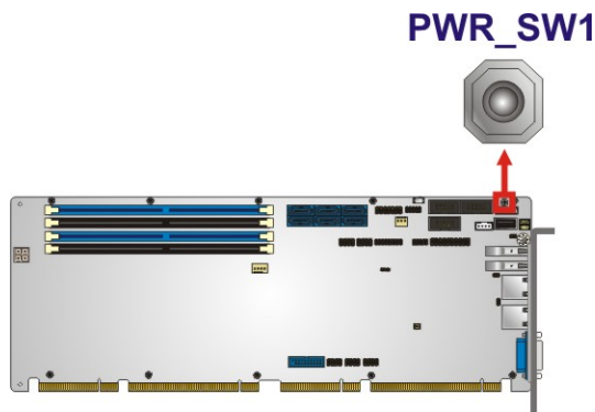
Figure 3-16: Power Button Location
