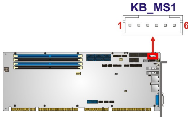
Figure 3-13: Keyboard and Mouse Connector Location
