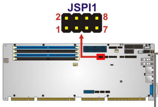
Figure 3-21: SPI Flash Connector Location
