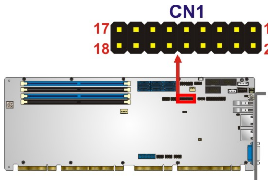
Figure 3-8: EC Debug Connector Location
