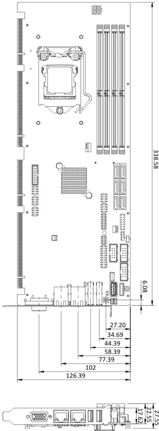
Figure 1-3: PCIE-Q370 Dimensions (mm)
