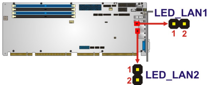
Figure 3-14: LAN LED Connector Locations
