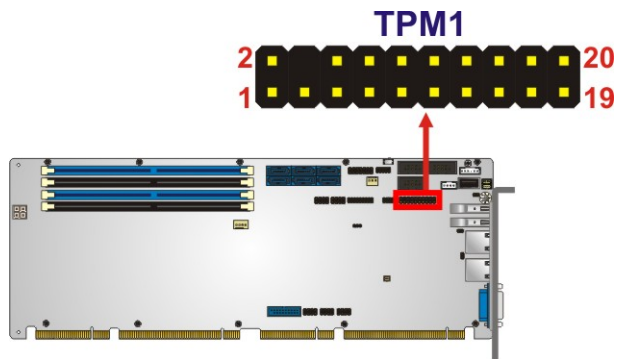
Figure 3-23: TPM Connector Location
