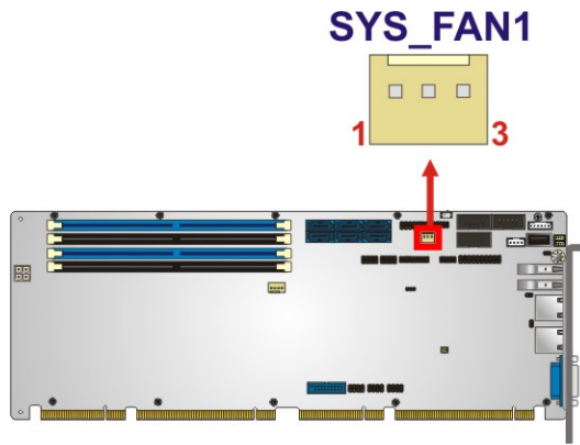
Figure 3-10: System Fan Connector Location
