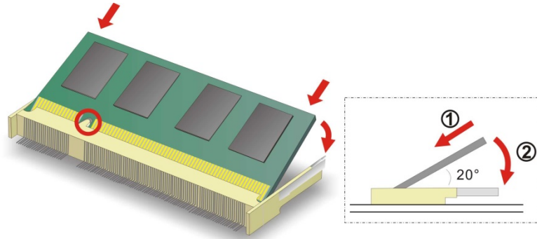
Figure 4-1: SO-DIMM Installation
