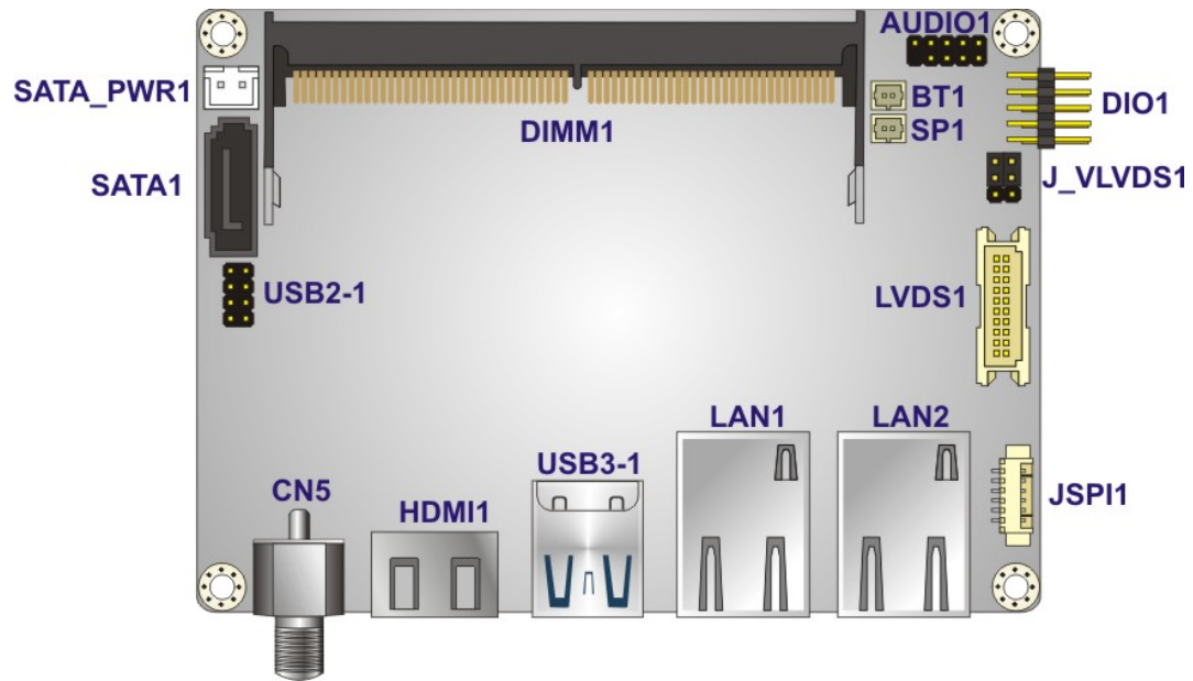
Figure 3-1: Connector and Jumper Locations (Front Side)
