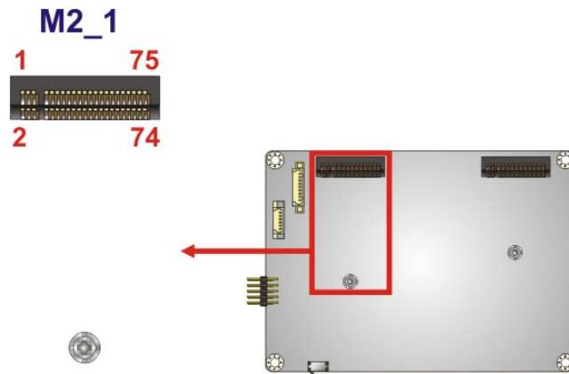
Figure 3-12: M.2 B-key Slot Location
