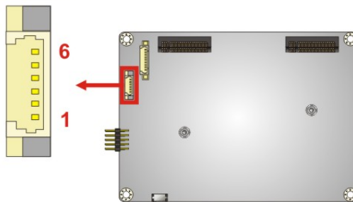
Figure 3-10: Backlight Inverter Connector Location
