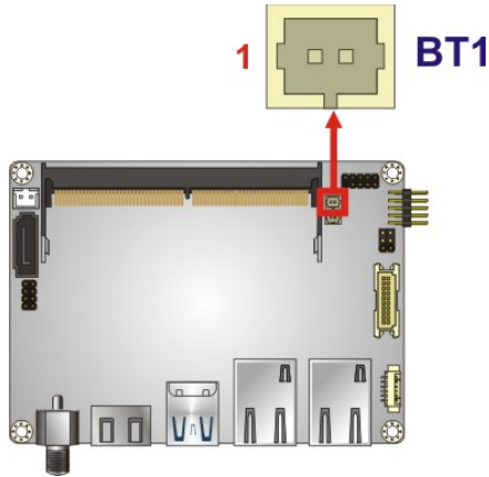
Figure 3-4: Battery Connector Location
