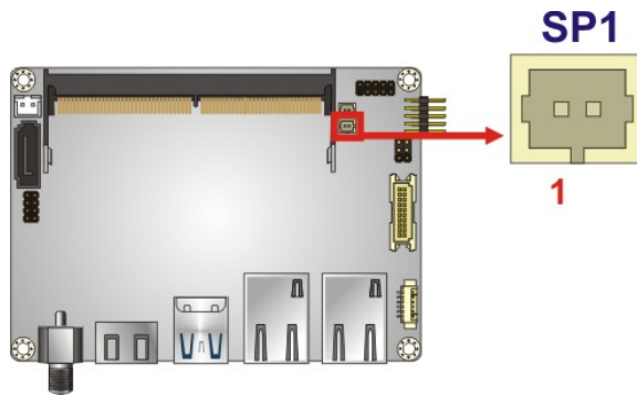
Figure 3-5: Buzzer Connector Location
