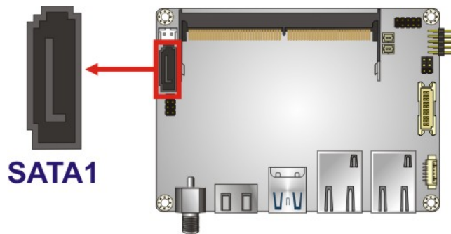
Figure 3-14: SATA 6Gb/s Connector Location
