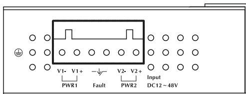
Figure 2-4 Industrial Media Converter Upper Panel.
