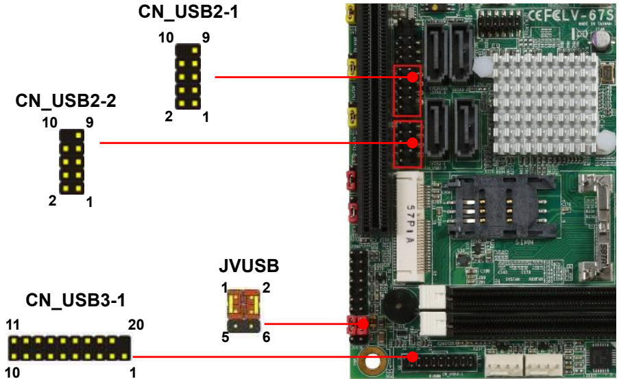
CN_USB 2-1/2-2: USB2.0 10-pin header (Pitch 2.54 mm)
