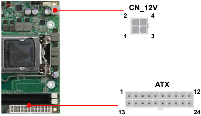
CN_12V: ATX12V 4-pin connector
