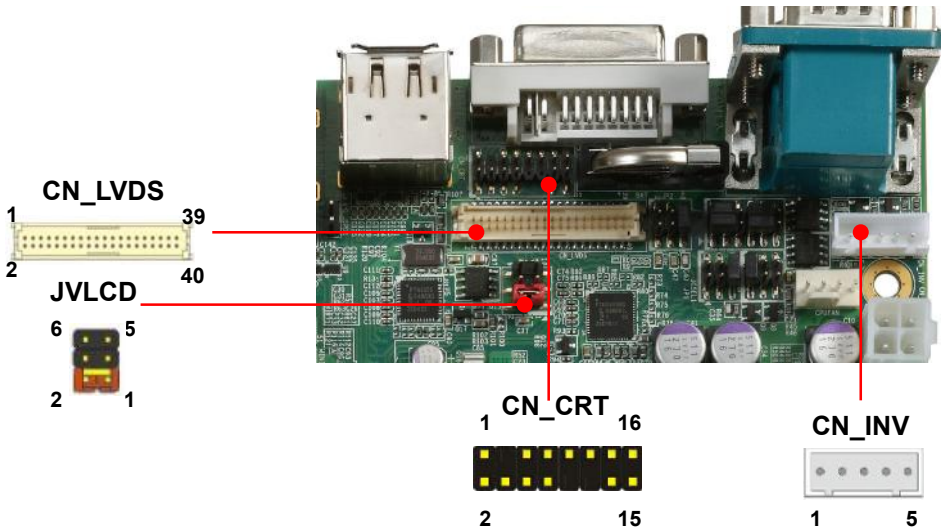
CN_CRT : CRT 16-pin connector (Pitch 2.00 mm)
