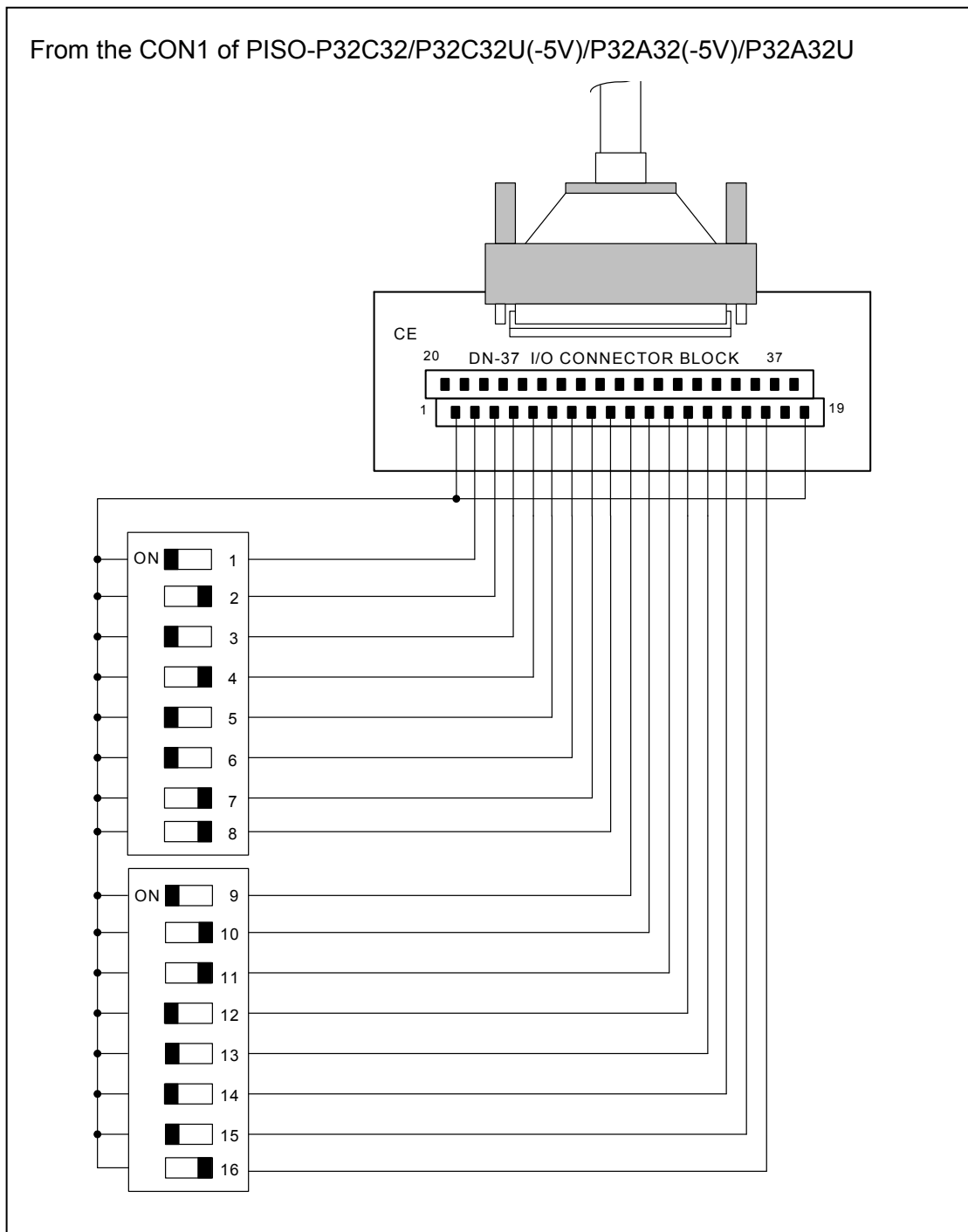
Figure 4-1-6. The circuit diagram of external device 1 for the DI of PISO-P32C32/P32A32(-5V)/P32A32U
