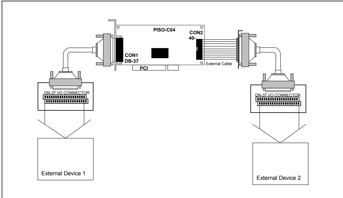
Figure 4-3-1. The example of digital outputs for PISO-C64(U)/A64
