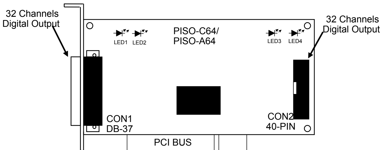
Figure 2-1A. Board layout of PISO-C64/A64
