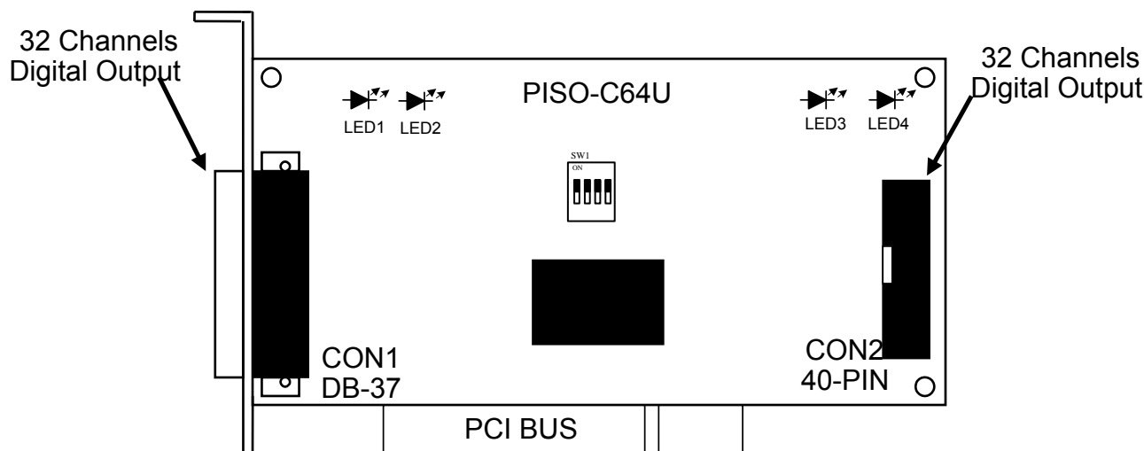
Figure 2-1B. Board layout of PISO-C64U
