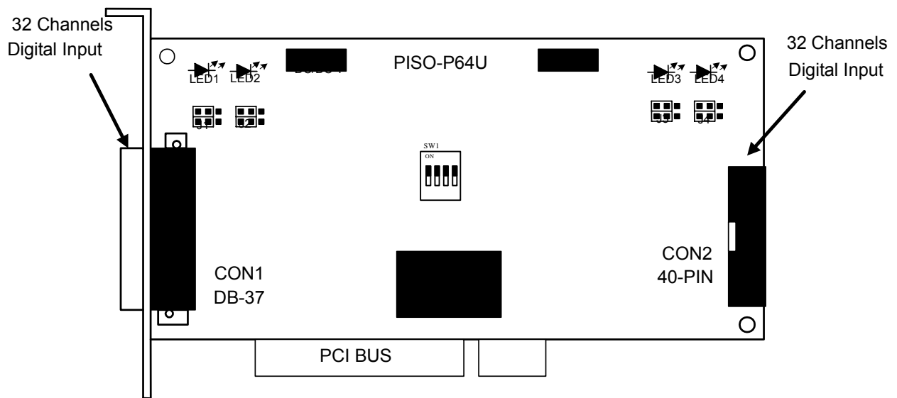
Figure 2-1B. Board layout of PISO-P64U
