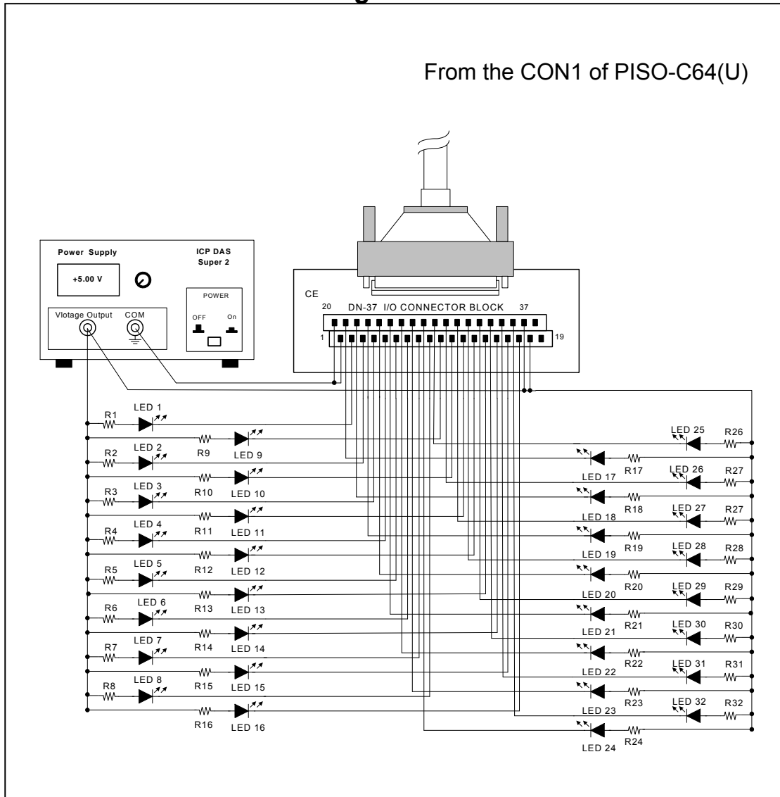
Figure 4-3-2. The circuit diagram of external device 1 for the digital outputs of PISO-C64(U)
