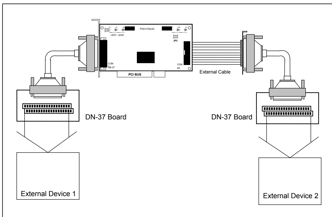
Figure 4-1-1. Digital inputs/outputs for PISO-P32C32/P32C32U(-5V)/ P32S32WU/P32A32(-5V)/P32A32U
