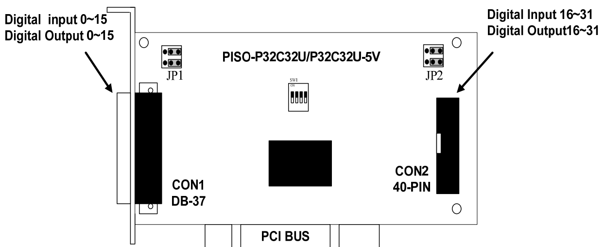
Figure 2-1B. Board layout of PISO-P32C32U/P32C32U-5V
