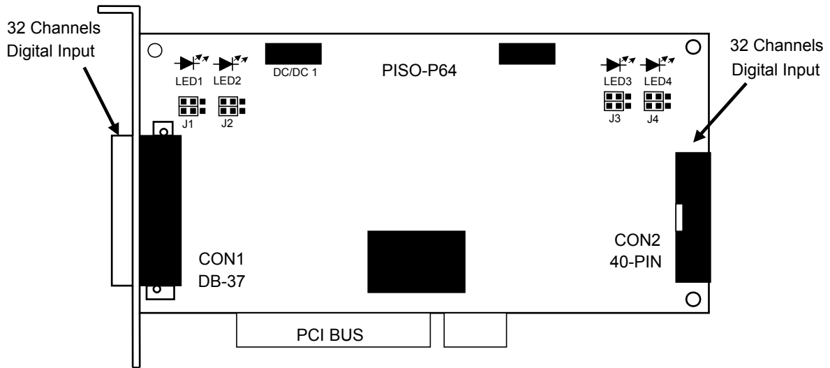
Figure 2-1A. Board layout of PISO-P64
