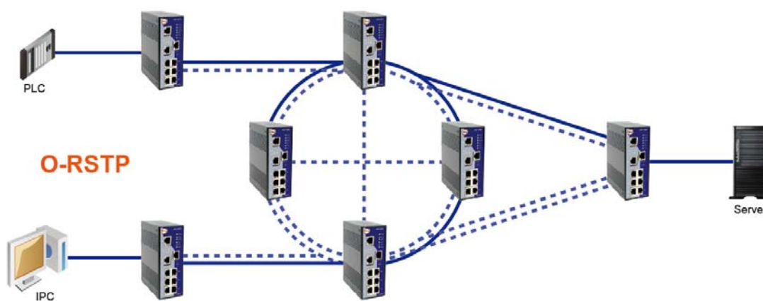
O-RSTP connection
