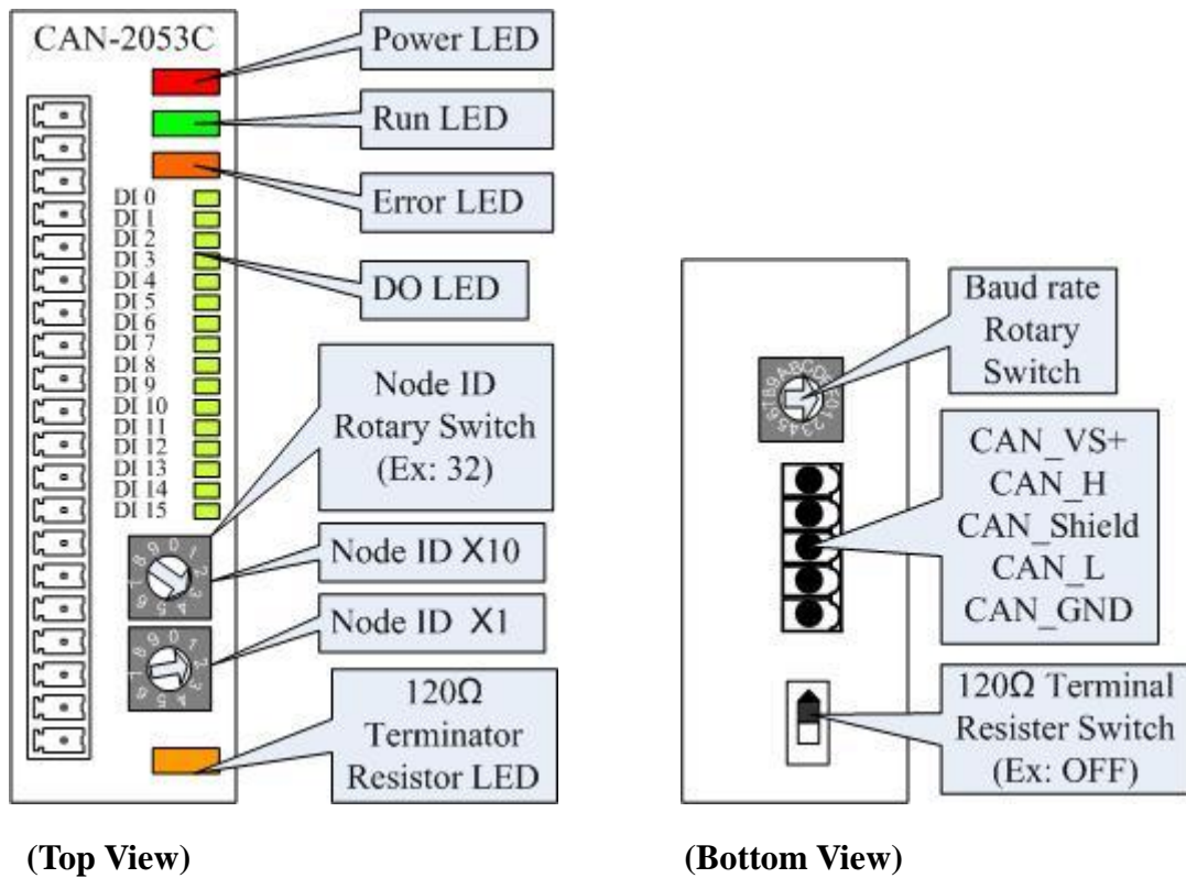
Figure 2-1 CAN-2053C layout of LED, connect, and switch
