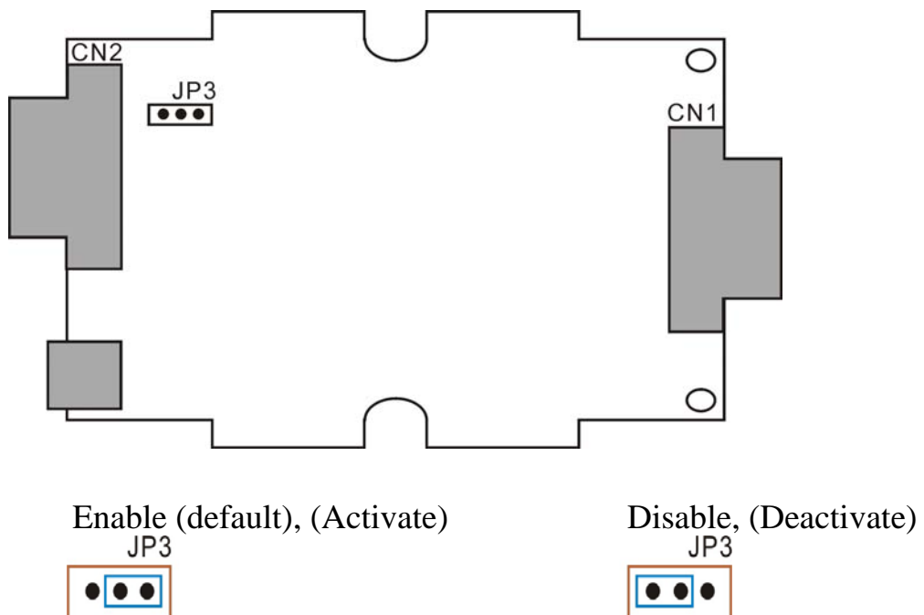
Figure 6: JP3 positions
