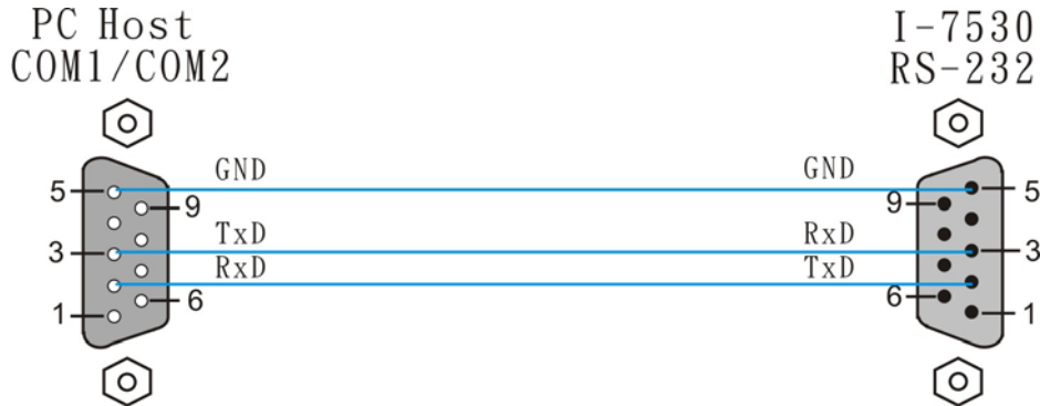
Figure 3: RS-232 connection
