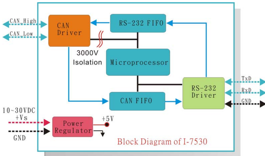
Figure 1: Block diagram of I-7530
