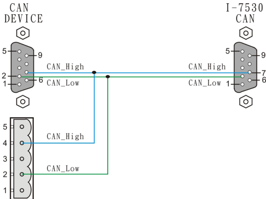
Figure 4: CAN connection
