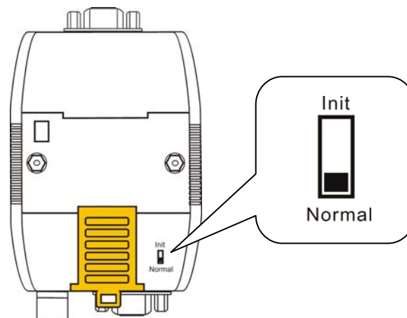
Figure 7: Dip-switch of I-7530
